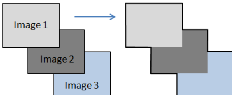
Figure 3: Image Mosaicking
