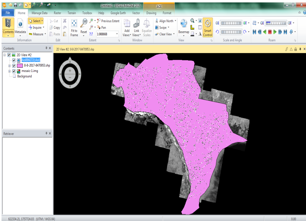
Figure 11: Habitation/ Urbanization in Krishna District
