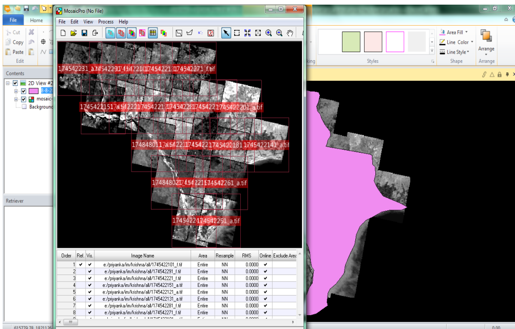
Figure 5: Non mosaicked Scenes
