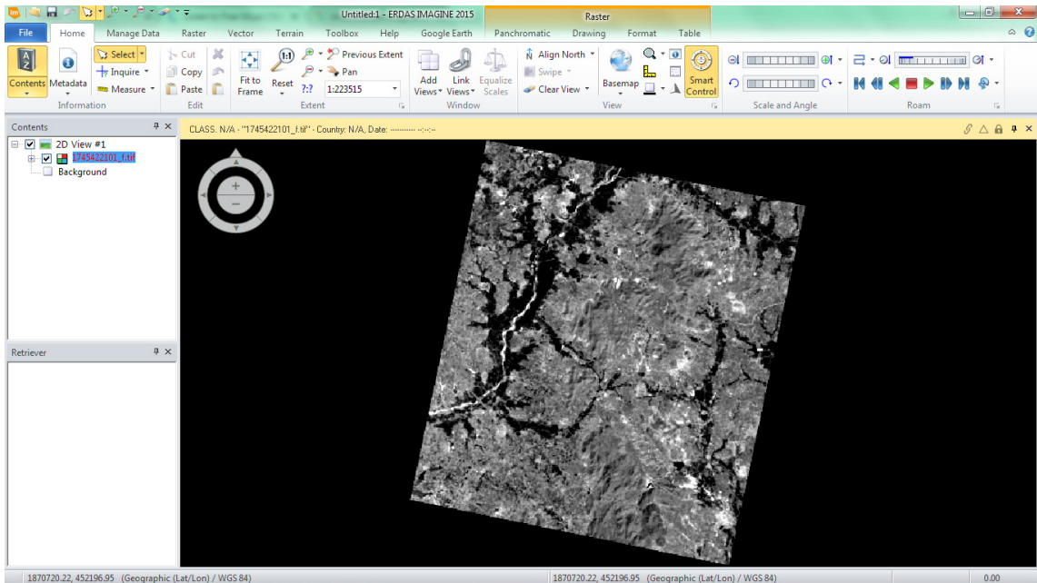
Figure 4: Individual Scene/Image
