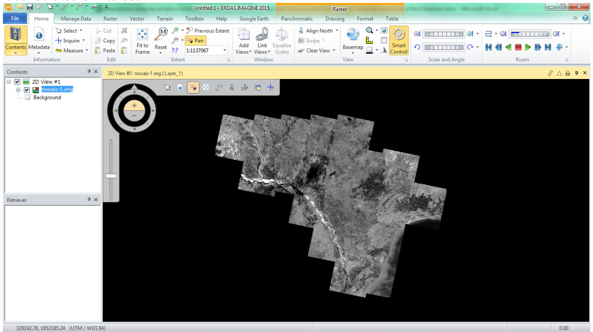
Figure 6: Mosaicked Scenes
