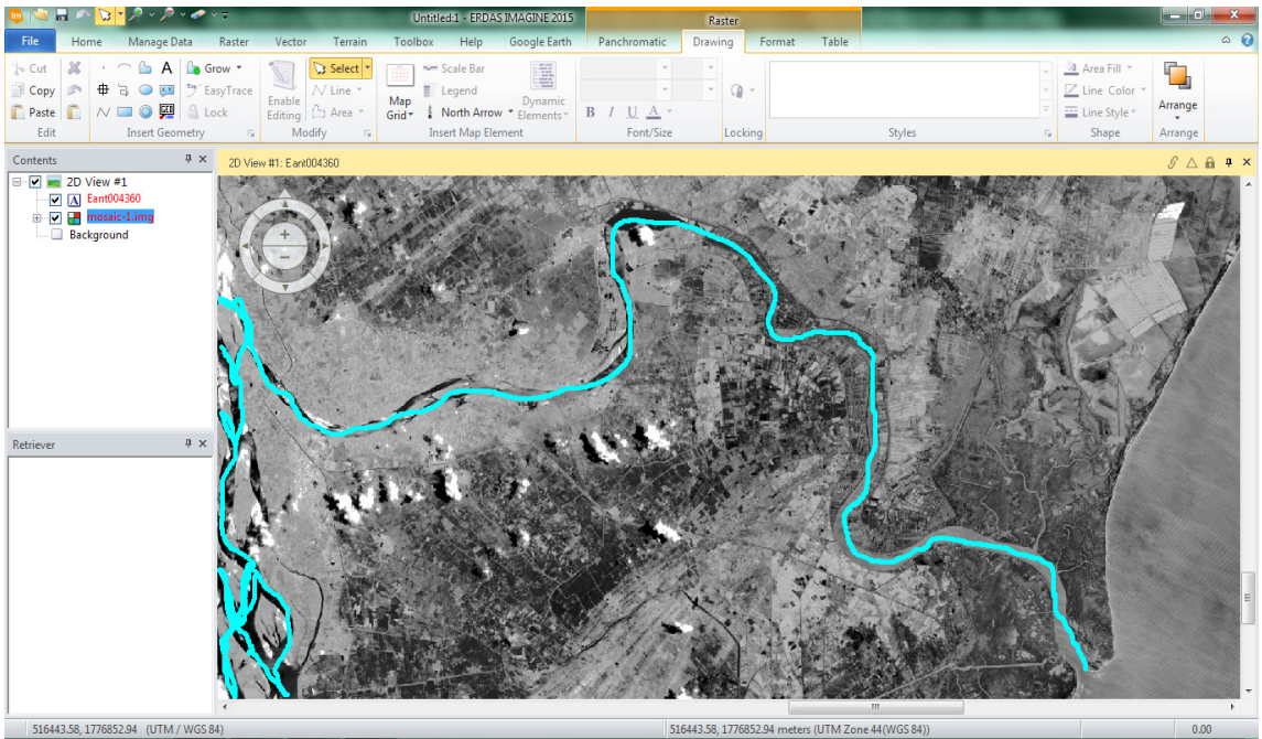
Figure 8: free hand polyline used to mark the river
