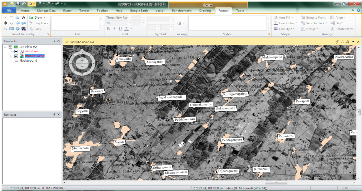
Figure 12: Identified area tagged with name (City, Town, and Village)
